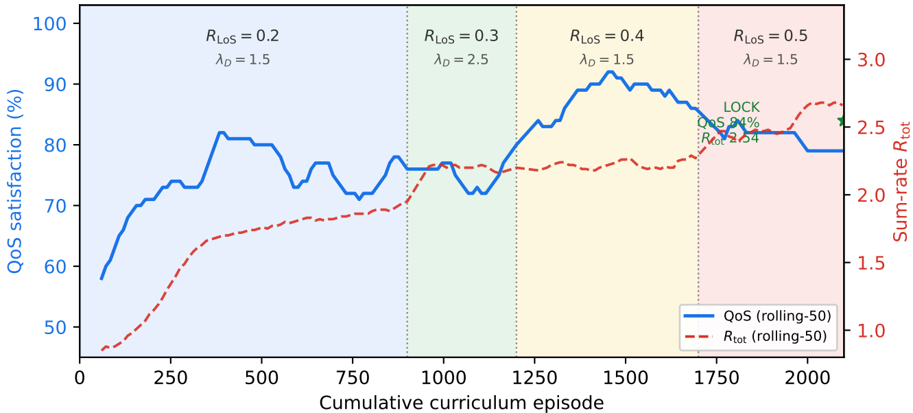
Case 1 ( K=5 , M=1 ) curriculum: QoS held across LoS-radius ramp 0.2 \rightarrow 0.5
